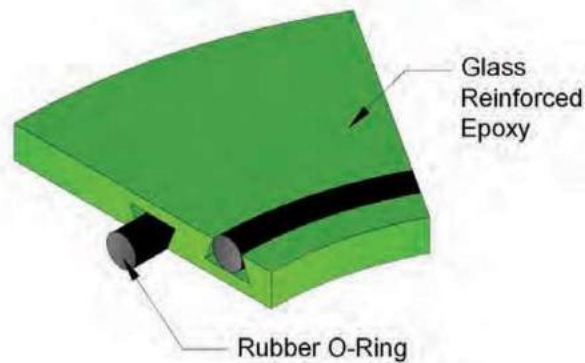
Picture 1. STARTEC® 9230-ES Cross Section
